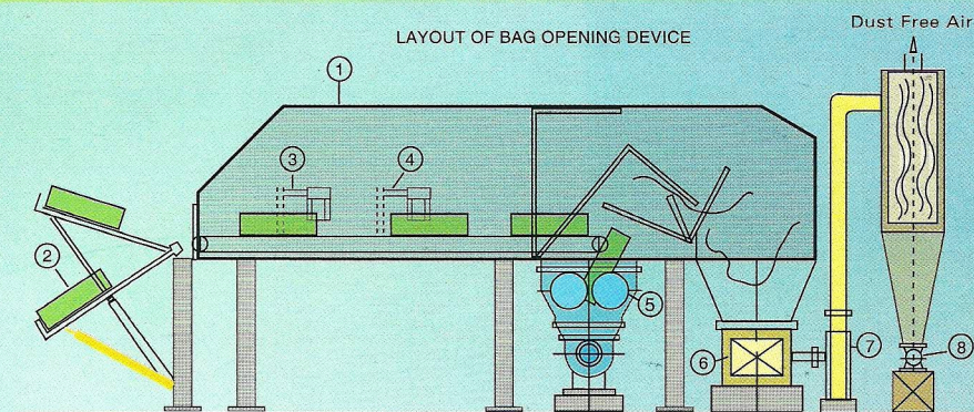
LAYOUT OF BAG OPENING DEVICE
